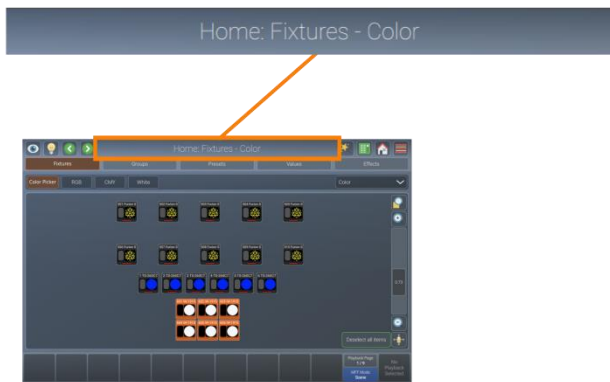
Fig. 13: Window Title
