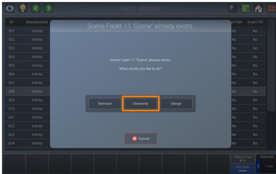
Fig. 159: Scene – Overwrite
